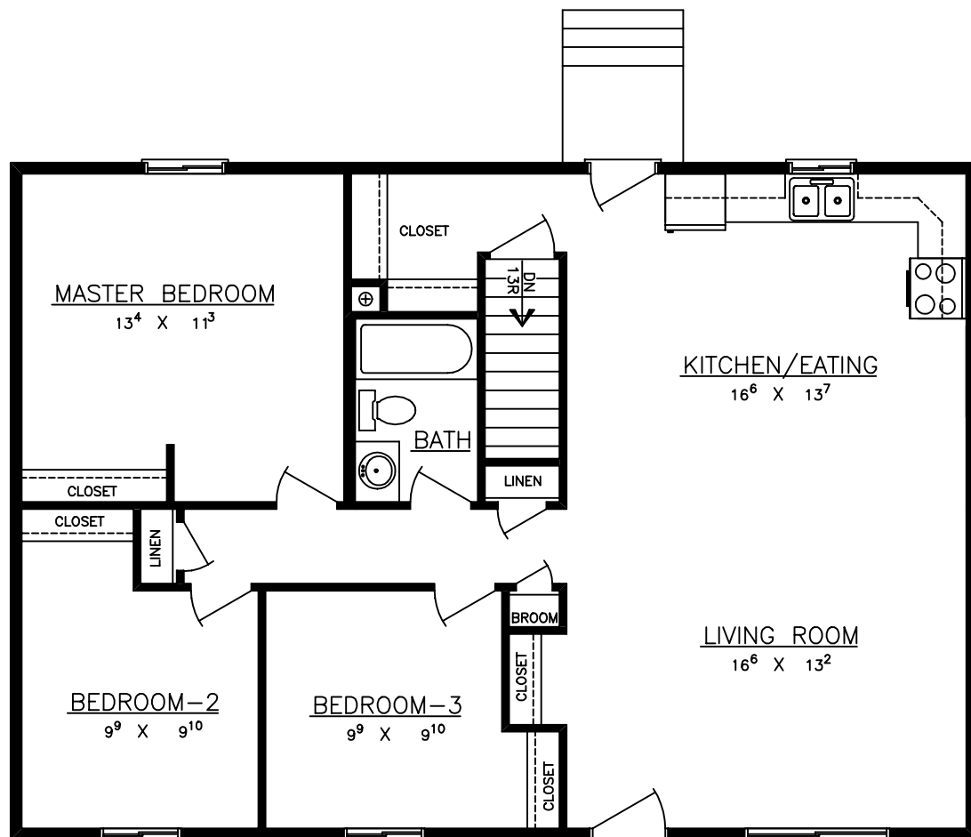
FLOOR PLAN
